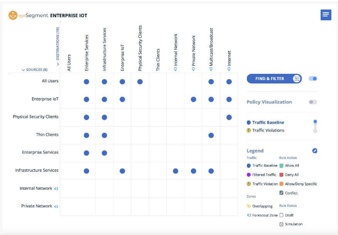
Figure 2. The eyeSegment Matrix allows you to focus on what is important. For instance, you can analyze and investigate a particular traffic pattern in your environment, as shown above. No matter where you are in the matrix hierarchy, you can instantly create and monitor effective eyeSegment policies to segment a specific traffic pattern and protect the EoT while ensuring business continuity.
