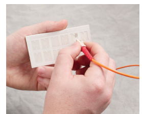
The right tools will help with fiber end face cleaning. Solvent from a fiber optic solvent pen, applied to a special purpose, disposable cleaning pad, is a best-practice method cleaning fiber optic cabling.
